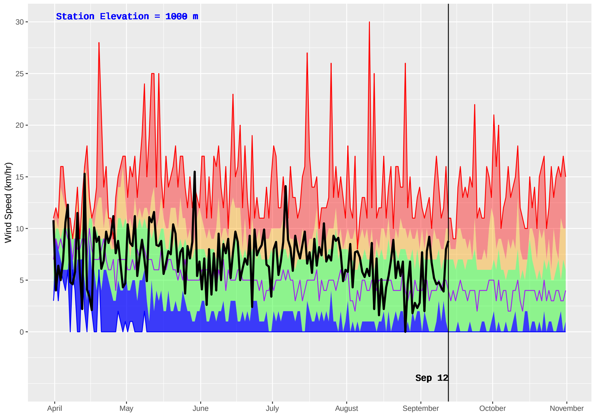
SUCCOUR CREEK (374) : Historical (1986–2016) and Current (2018) Daily Wind Speed
