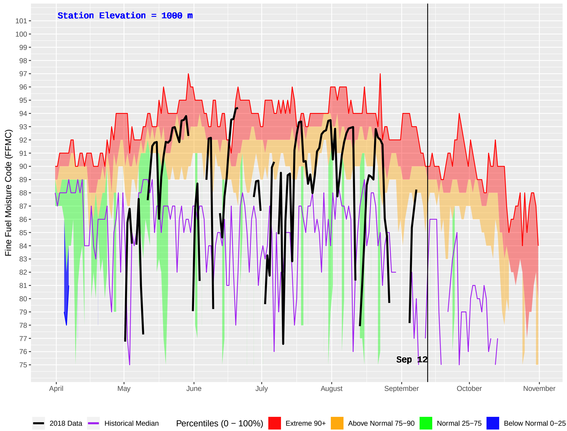
SUCCOUR CREEK (374) : Historical (1986–2016) and Current (2018) Daily Fine Fuel Moisture Code (FFMC)
